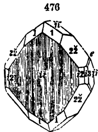
Norway, Me.
